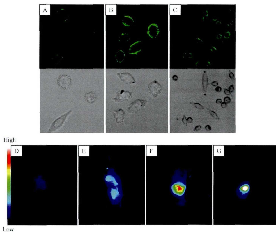
Fig. 4 Temporal internalization of L-QD by confocal microscopy and NIR images. Confocal microscopy images of MCF-7 cells incubation with lipid-QD after different time, top panel-fluorescence channel, bottom panel-bright-field. A: lipid-CdTe 30 minutes. B: lipid-CdTe 60 minutes. C: lipid-CdTe 120 minutes. D-G represent NIR images of the denuded mouse after lipid-CdHgTe was injected via tail vein for 10 seconds, 5, 10, and 20 minutes, respectively. Reproduced with permission from ref. 67. Copyright 2013 Springer.
